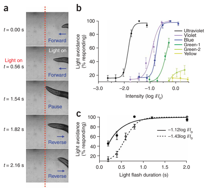
Figure 1 Light evokes avoidance responses in C. elegans in a dose-dependent manner. (a) Snapshot images showing that a flash of light triggered an avoidance response in a worm moving forward. A flash of light (2 s, UV-A) was delivered by an objective to the head of a worm moving forward under a microscope. The animal quickly responded by stopping forward movement and initiating reversals. The dotted red line indicates the position of the worm in the field. (b) Worms responded to light in an intensity-dependent manner and were most sensitive to UV-A light. Light pulses (2 s) of varying intensity were tested for the head avoidance response and the percentage of worms that responded was scored ( I_0 = 20 \text{ mW mm}^{-2} , n = 10 ). Error bars represent s.e.m. (c) Worms responded to light in a duration-dependent manner. Light pulses of varying duration were tested for the head avoidance response. Two different intensities of UV-A light were tested ( -1.12 \log I/I_0 and -1.43 \log I/I_0 , n = 10 ). We also examined violet and blue light ( Supplementary Fig. 1 ). Error bars represent s.e.m.
